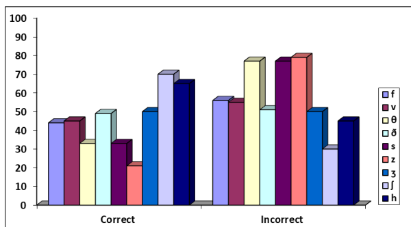
Fig 2: fricatives phonemes
