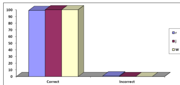
Fig 6: Approximate Phonemes
