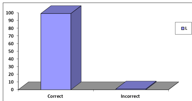
Fig 5: Lateral Phoneme
