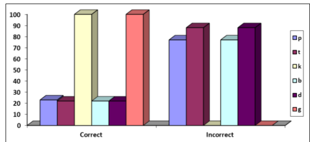
Fig 1: Plosive Phoneme
